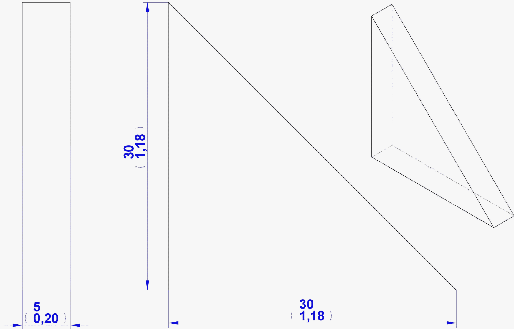
1.08 Triangle Support
