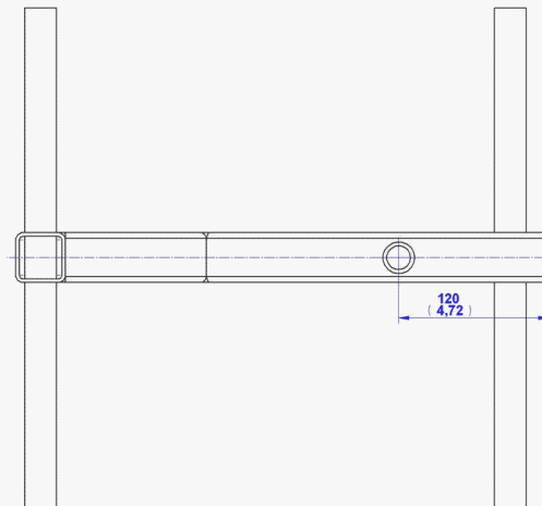
FRAME COMPONENTS 4.03, 4.04, 4.05, 4.06, 4.07, 4.08, 4.09
